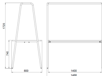
FourReal® A 90, 140 x 80 cm
