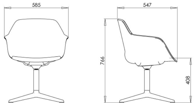
FourMe Lounge - Plastic shell - Inner upholstered - tilt - return
