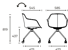
FourMe® 11 Polypropylene shell with castors
